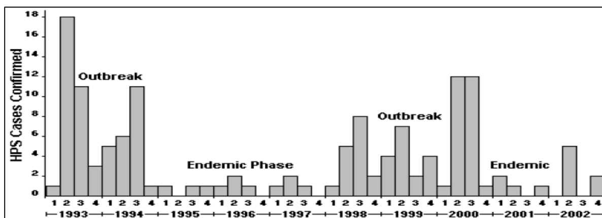
Figure 7. Cases of Hantavirus Pulmonary Syndrome (HPS) confirmed in the Four Corners states (Arizona, Colorado, New Mexico, Utah) from 1993 through 2002 by quarter of onset of symptoms. From "Hantavirus in Indian Country: The First Decade in Review," by R. Pottinger, 2005, American Indian Culture and Research Journal , 29(2), p. 42. Used with permission of the author.
